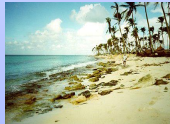
Gran Dominicus Resort, Dominican Republic. Before and after construction of Reef Ball Breakwater, 1998 and 2001. Sand accreted at a rate of 26-44 m 3 /m from 1998-2001. Photo: Lee Harris
